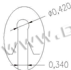
2, 5, 8, 11, 16线槽
